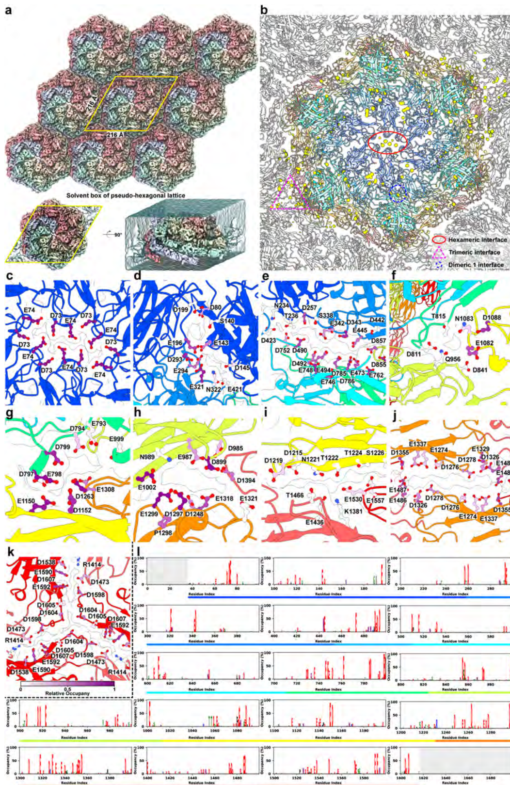
Extended Data Fig. 6 | Molecular dynamics simulation of ammonium ion diffusion across the multi-channel, charged S-layer. a , Unit cell design for MD simulation of the S-layer lattice. The unit cell (simulation box, outlined in yellow) was constructed to simulate an infinite two-dimensional sheet. b , Ammonium ion density (ammonium occupancy during a single simulation shown as golden density) plotted onto the structure shown in ribbon representation. For further details on ammonium binding residues, please see Supplementary Table 2 and
