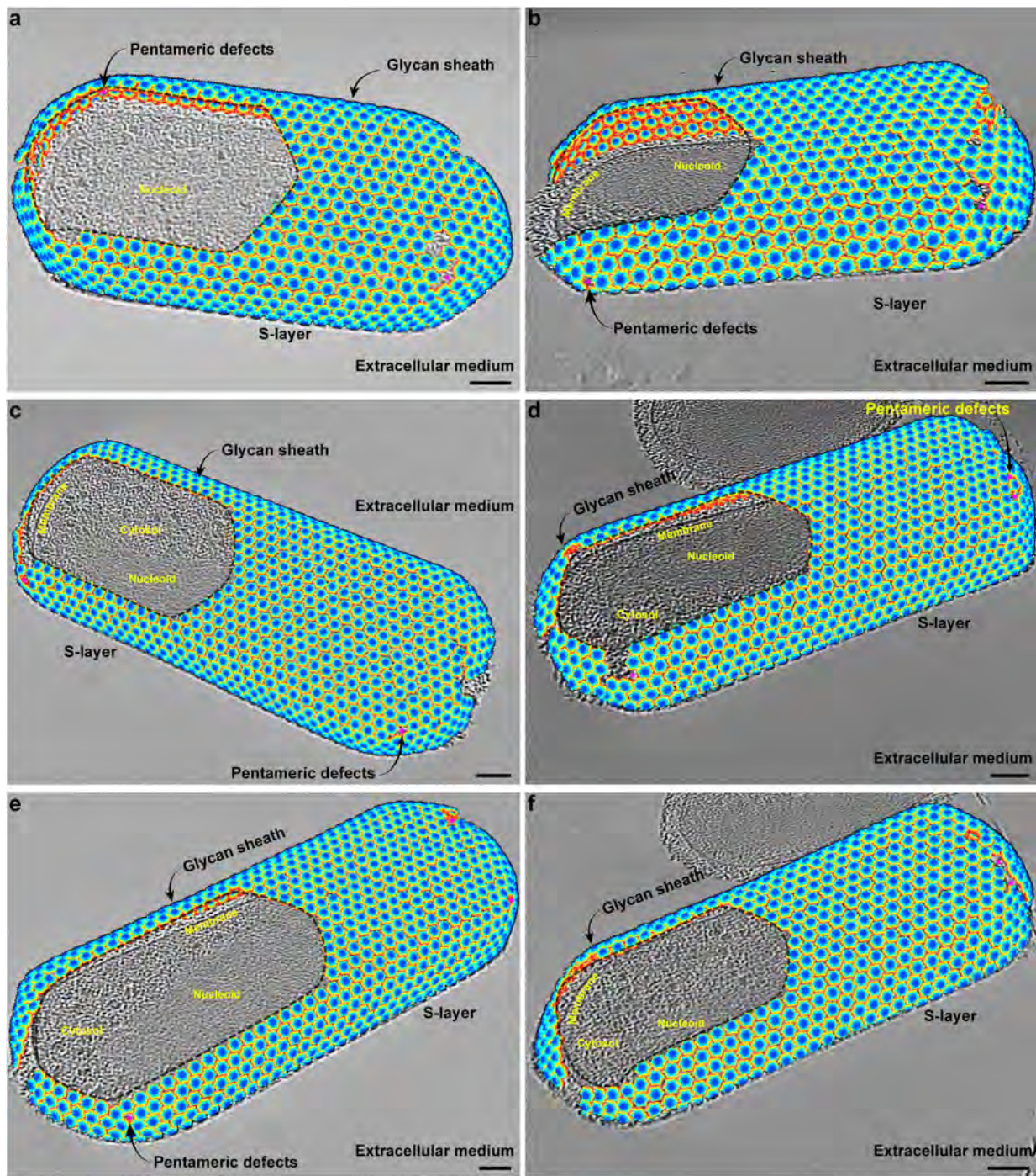
Extended Data Fig. 8 | Whole cell tomography of N. maritimus and S-layer lattice maps. a-f, Gallery of lattice maps of the S-layer from subtomogram averaging plotted onto denoised 36,37 N. maritimus cellular tomograms (only one slice shown in each case). The S-layer lattice coats nearly the entire outer surface of N. maritimus cells. A region has been cut out from each lattice map
